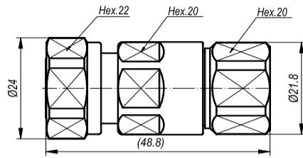
4.3-10 Straight male Connector for 1/2" Flexible RF Cable
